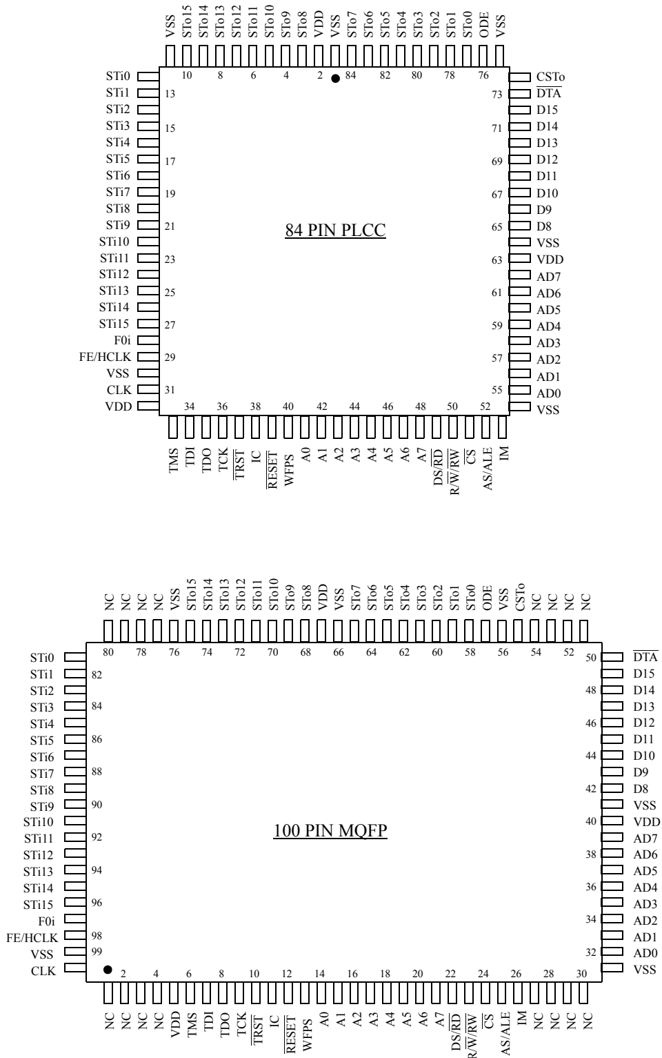
Figure 2 - Pin Connections
